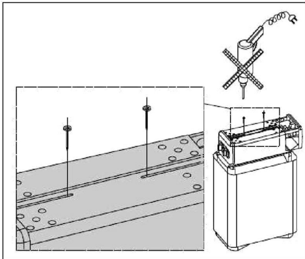
Figure 6. Removal of the end-piece fastening screws
